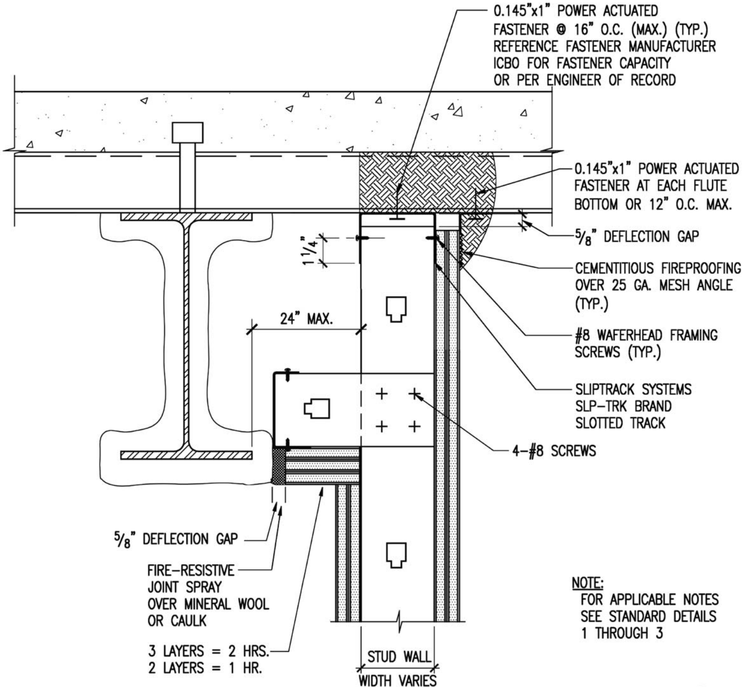
HEAD OF WALL PARALLEL TO BEAM — OPTIONAL SYSTEM 6 FIRE RATED DESIGN UL-2079 TEST STD.
