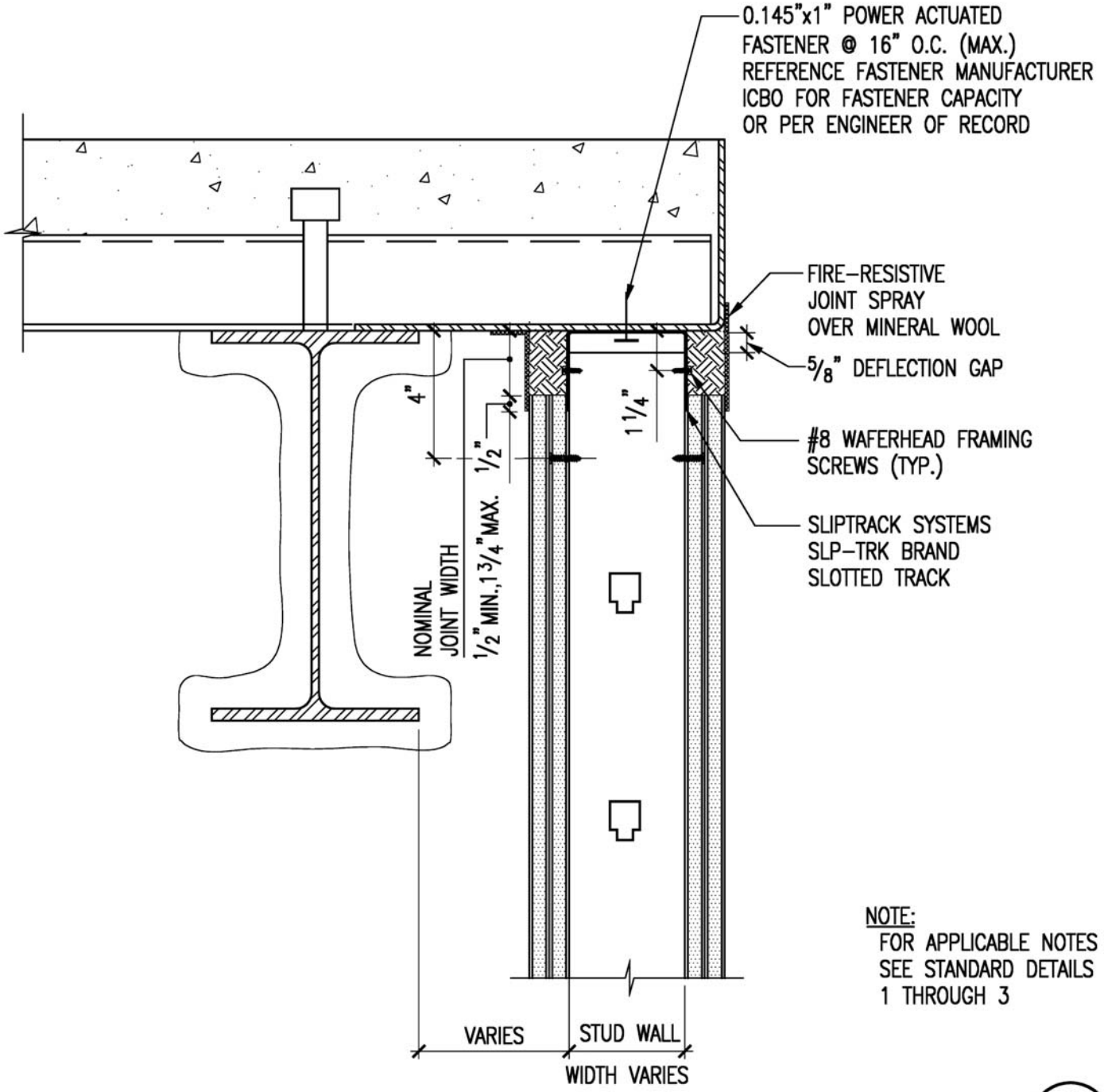
HEAD OF WALL AT SLAB EDGE SYSTEM 7-19 FIRE RATED DESIGN UL-2079 TEST STD.
